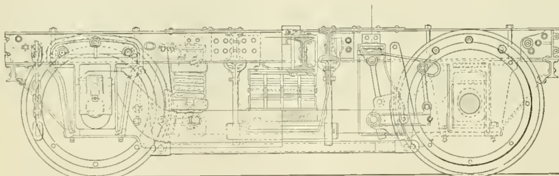
STEEL FRAME PASSENGER CAR TRUCK—L. S. & M. S. RY.
